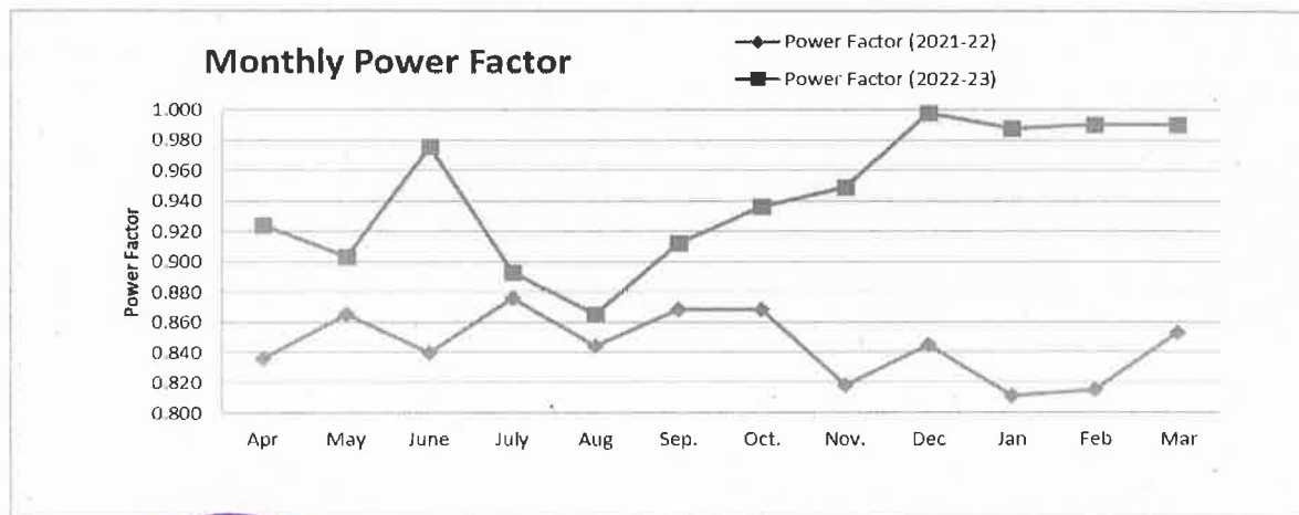
Fig.3.4 Monthly Power Factor for the year (2021-22) and year (2022-23)
