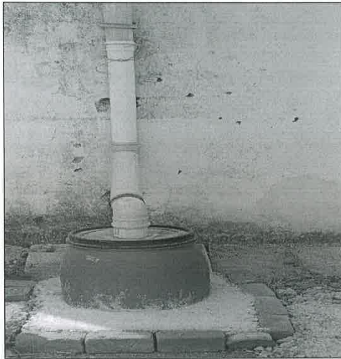
Figure: - 4.1 Rainwater harvesting in institute
