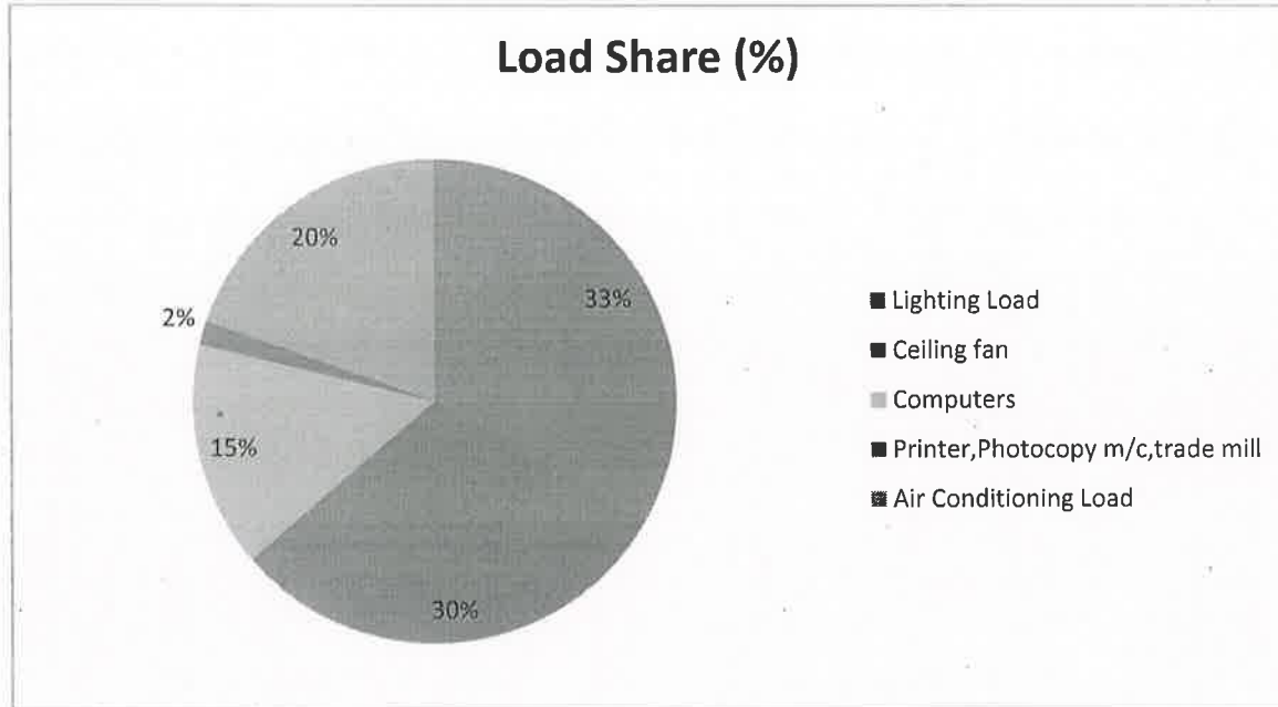
Fig.4.1: Load Share of the TIT Excellence Building
